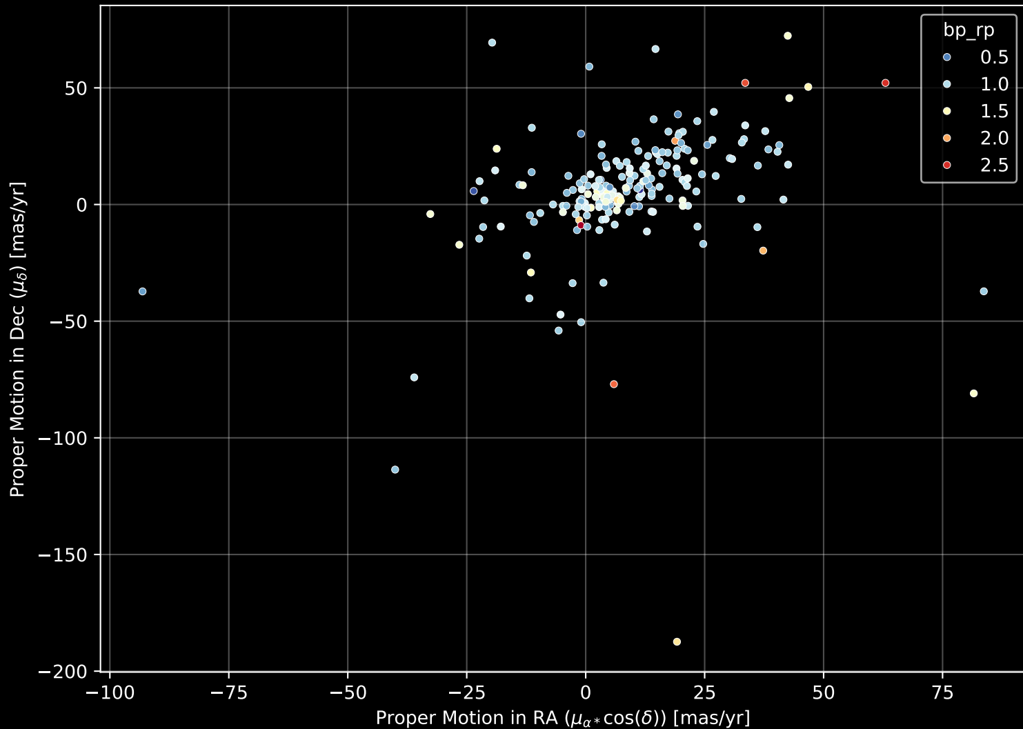
APOGEE DR17 Field: [284-40-O_TESS] Proper Motion Diagram (n= 198)
