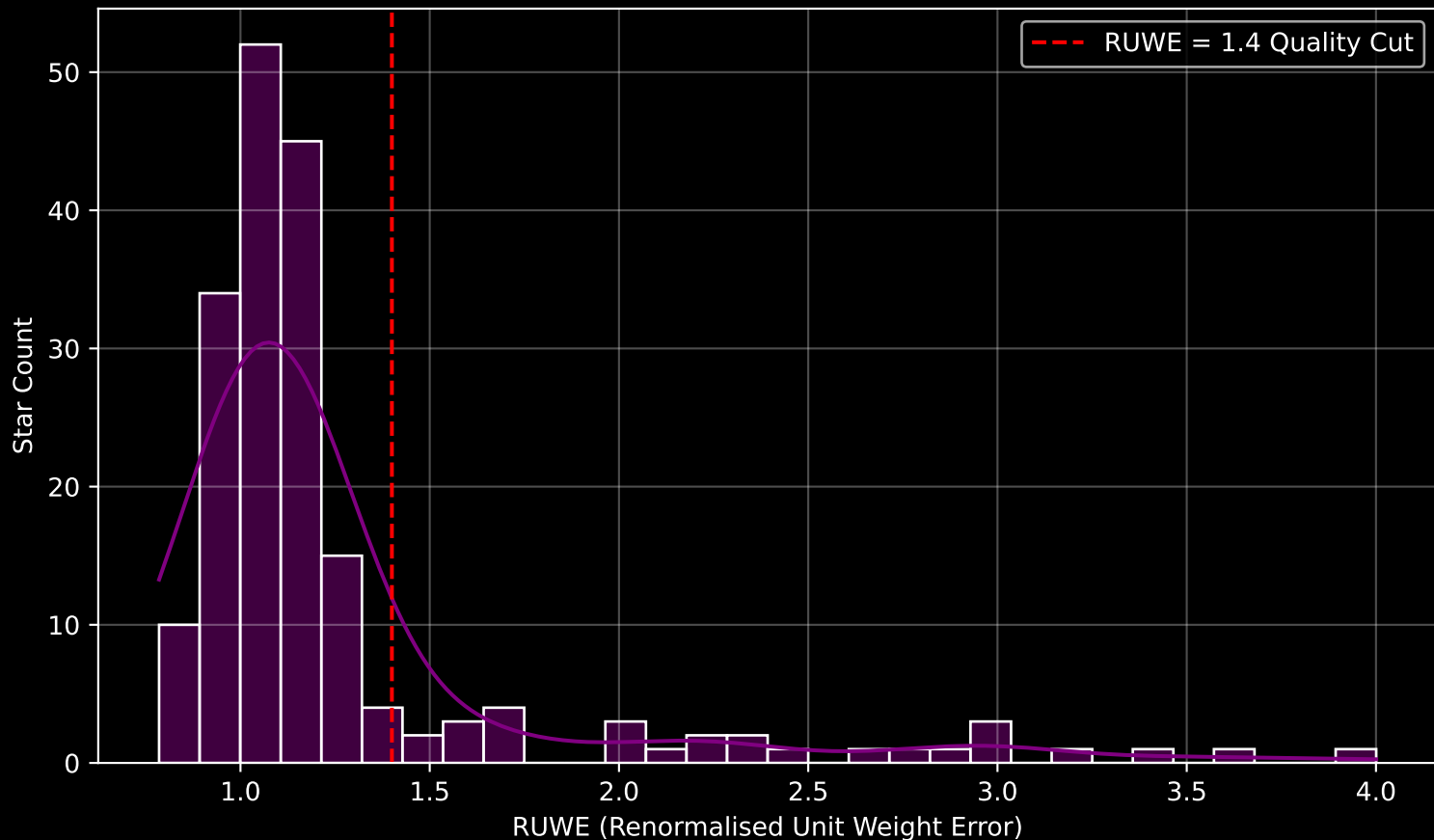
GAPOGEE DR17 Field [284-40-O_TESS] RUWE Distribution (n= 188)
