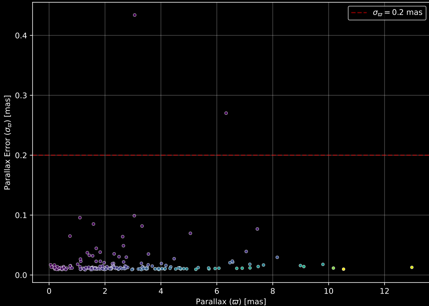
APOGEE DR17 Field: [284-40-O_TESS] Parallax Quality (n= 198)
