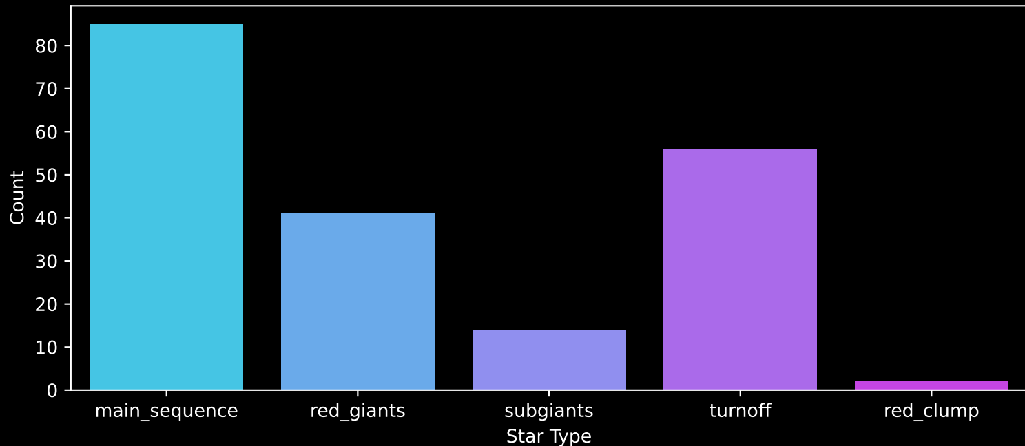
APOGEE DR17 Field: [284-40-O_TESS] Count plot of Star Type
